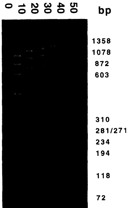
Figure 3a. (a) Effect of ligand binding on the electrophoretic mobility of \phi\text{X-174} DNA digested with endonuclease restriction fragments (sizes indicated to the right side of the figure). Lanes 1–6 have the indicated concentrations (in \mu\text{M} ) of 4 (0 is control DNA restriction fragments with no added agents).
