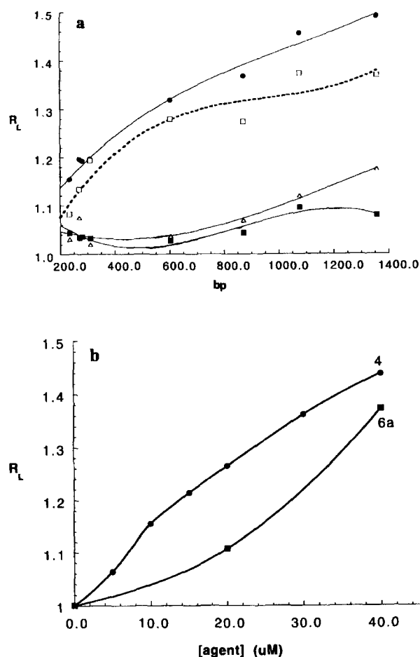
Figure 3b. (a) A plot of the ratio of apparent DNA length to real length ( R_L ) versus the number of base pairs (bp) in the longest and intermediate sized DNA fragments in the presence of 40 \mu\text{M} 4 ( \bullet ), 40 \mu\text{M} 6a ( \square ), 150 \mu\text{M} Dm ( \blacksquare ) and 150 \mu\text{M} 18 ( \triangle ). The curves are interpolations between the data points for 4 . (b) Employing the 1078 bp DNA fragment plot of the ratio of apparent DNA length to real length ( R_L ) versus [agent] [ 4 ( \bullet ), 6a ( \blacklozenge )]. The curves are interpolations between the data points for 4 and 6a . The data for Figure 3(b) was generated from Figure 3(a) and previously collected data 3d as explained in the text.
