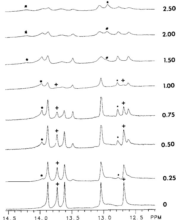
Figure 2. Titration of a solution 1 mM in d(CGCAAATTTGCG) 2 , 10 mM phosphate buffer (pH 7.0) with 4 in H 2 O:D 2 O 9:1 at 25 °C at the indicated mol ratios of 4 /dsDNA. The binding of 4 was followed by the disappearance of the resonances marked with plus (+) signs and the appearance of the resonances marked with asterisks (*) in the titration spectrum.
