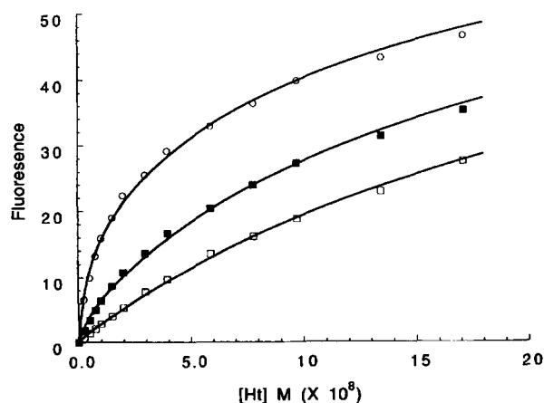
Figure 1. Representative plots of fluorescence ( F , in arbitrary units) versus total Hoechst 33258 ( Ht ) concentration at pH 7.0 and 35 °C for 4 at 5.0 \times 10^{-9} M (○), 7.5 \times 10^{-9} M (■) and 1.0 \times 10^{-8} M (□) in the presence of 5.0 \times 10^{-9} M d(GGCGCA 3 T 3 GGCGG)/d(CCGCCA 3 T 3 GCGCC). The theoretical curves which fit the points were computer generated by optimizing the constants in equation (1).
